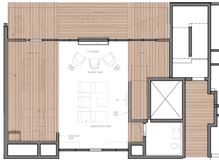
AMENITY ROOM RCP
